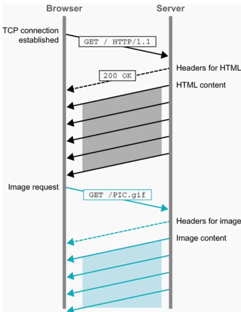
Figure 1.4 HTTP 1.1 transfers
