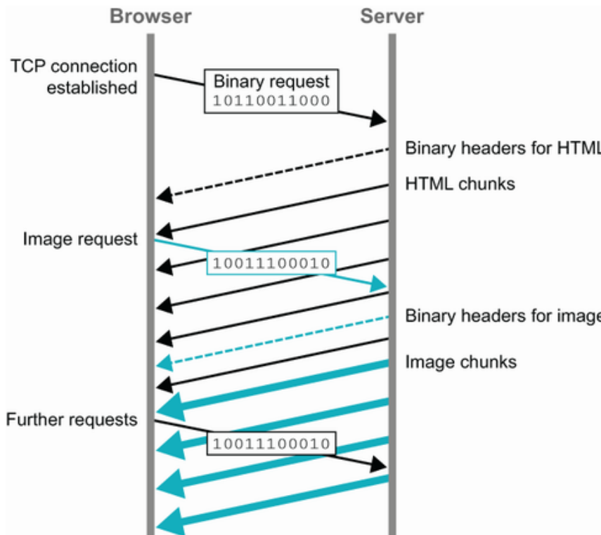
Figure 1.5 HTTP/2 transfers
